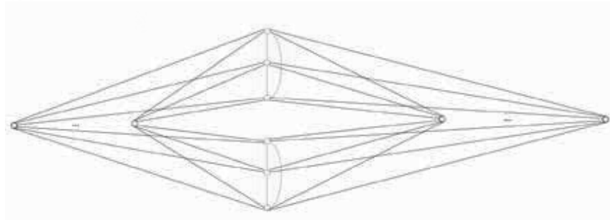
Drawing of G_1 + nK_1
