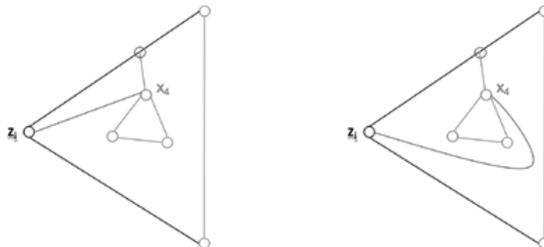
Tracing edges of G_2
