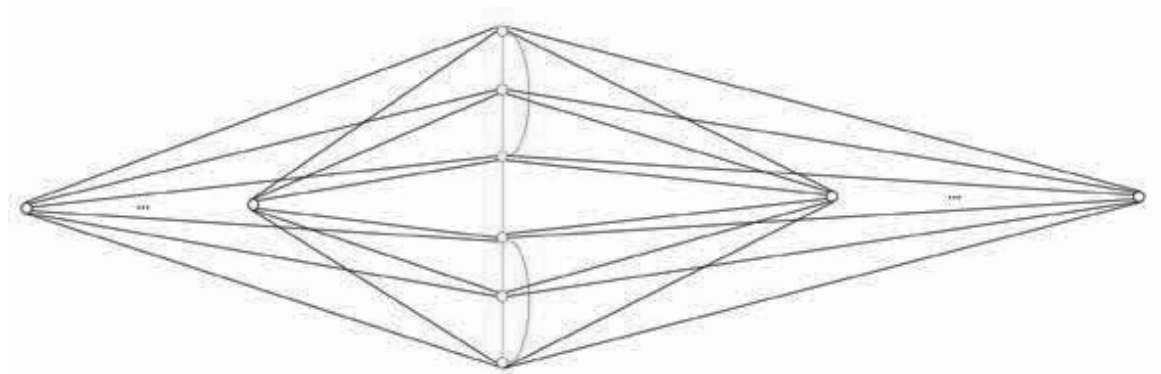
Drawing of G_2 + nK_1
