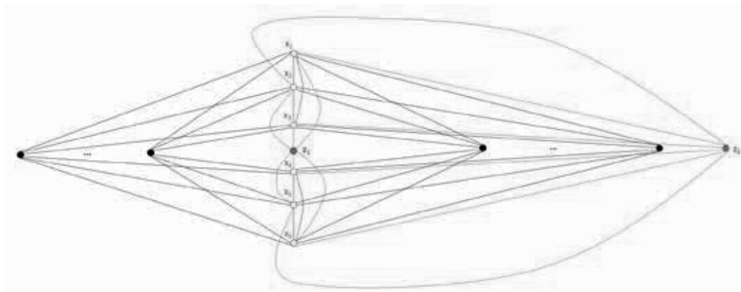
Drawing of G_1 + nK_1 for odd n
