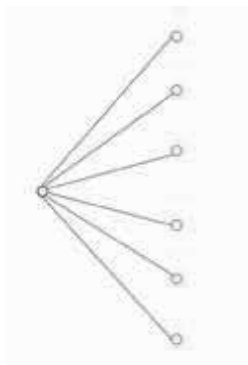
Drawing of T_i
