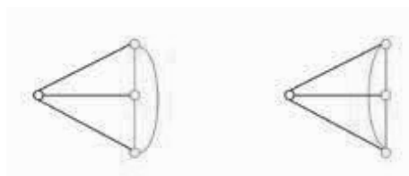
Drawings of one C_3 and z_i
